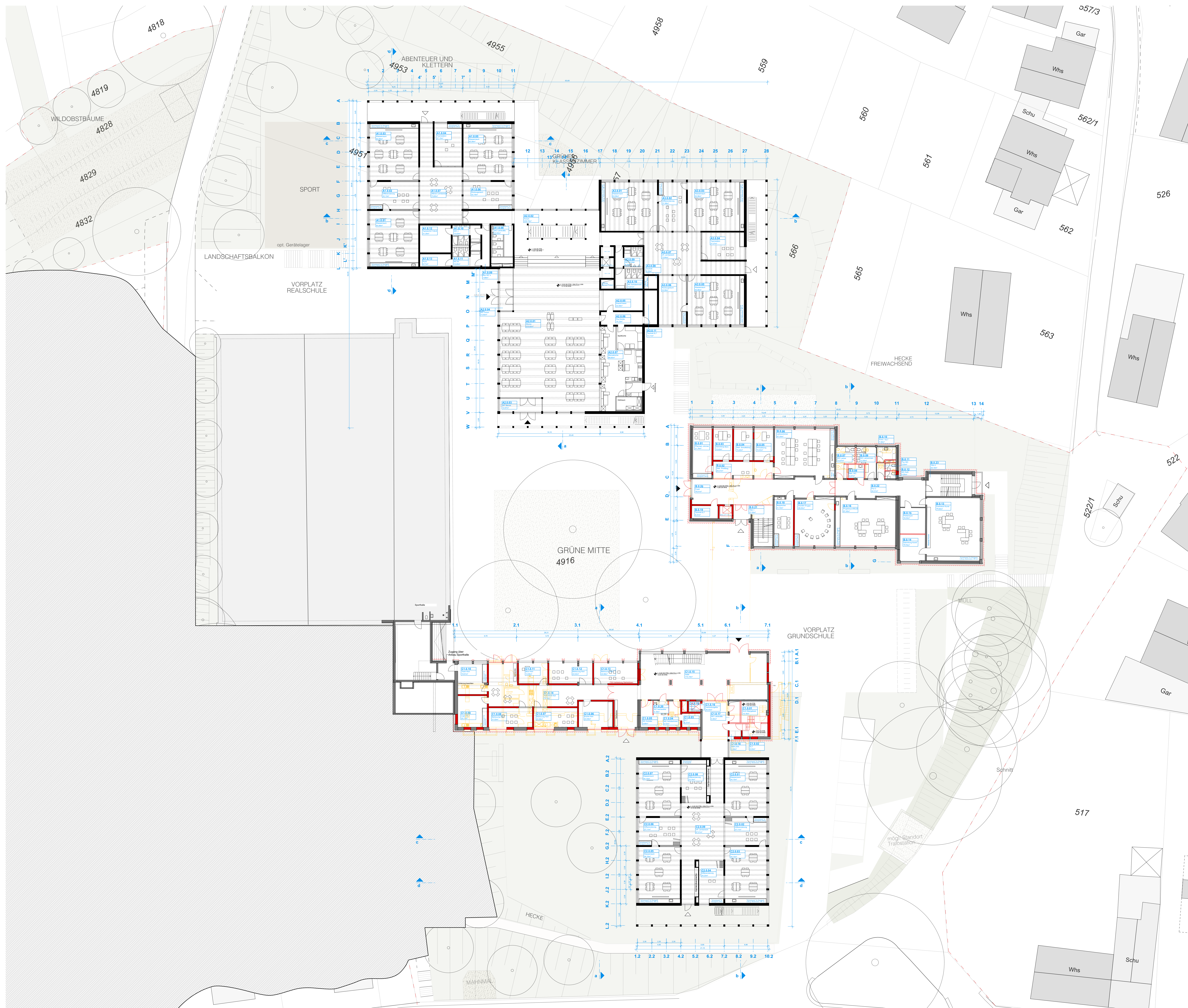
GRUNDRISS EBENE 0 ARC-XX-GR-E0-001-2
